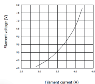
FILAMENT CHARACTERISTICS
