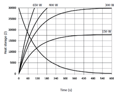
THERMAL CURVES
