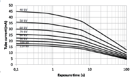
RATING CHARTS DC
