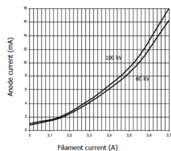
EMISSION CHARACTERISTICS DC
