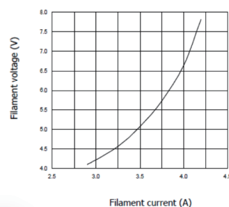
FILAMENT CHARACTERISTICS
