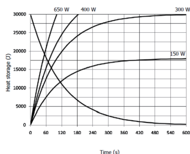
THERMAL CURVES
